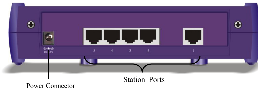
Fig. 2-3 Rear Panel
